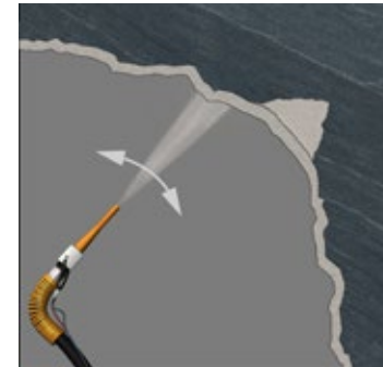
Fig. 7.3: 1st shotcrete layer – 1 st excavation stabilization and adhesive bridge for the 2 nd shotcrete layer
