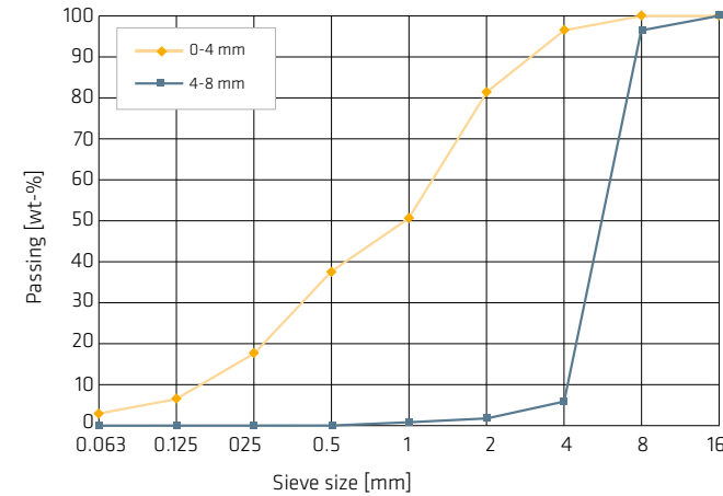
Fig. 5.5: Grading curves of the individual aggregate fractions
