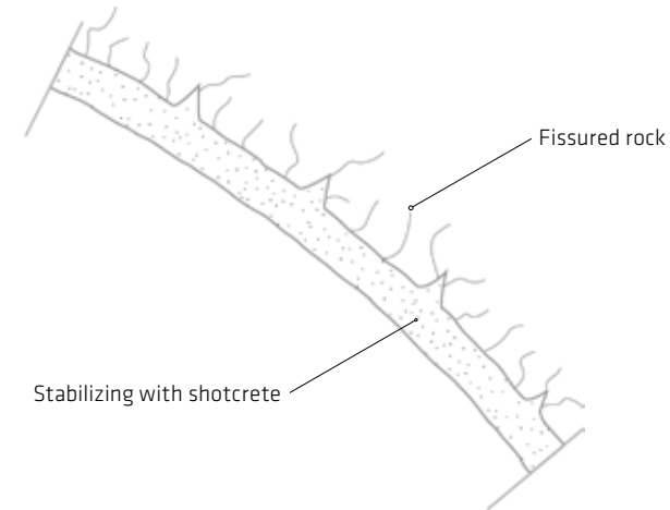
Fig 2.3: Stabilization by filling substrate cracks and building an arch of shotcrete and the surrounding rock
