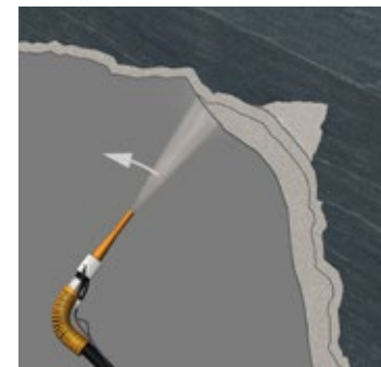
Fig. 7.5: 2 nd shotcrete layer – excavation stabilization, usually together with steel reinforcement
