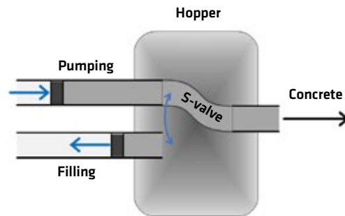
Fig. 6.2: Function principle of double piston pump
